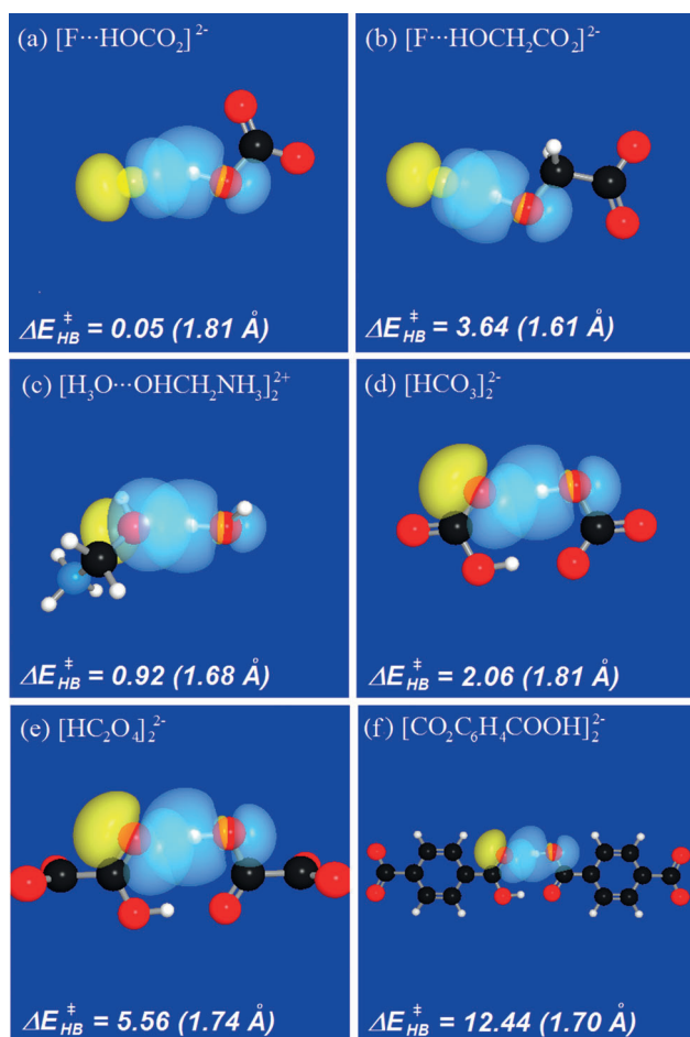
Figure 3. Optimized structures (with leading n_B \rightarrow \sigma_{AH}^* NBO interaction), H-bond well depths ( \Delta E_{HB}^{\ddagger} , kcal mol -1 ), and equilibrium R_{B...H} separations (in parentheses) for each AEHB species (a)–(f) discussed in the text.
